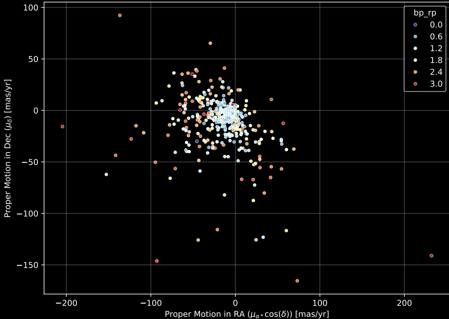
APOGEE DR17 Field: [300+75] Proper Motion Diagram (n= 410)
