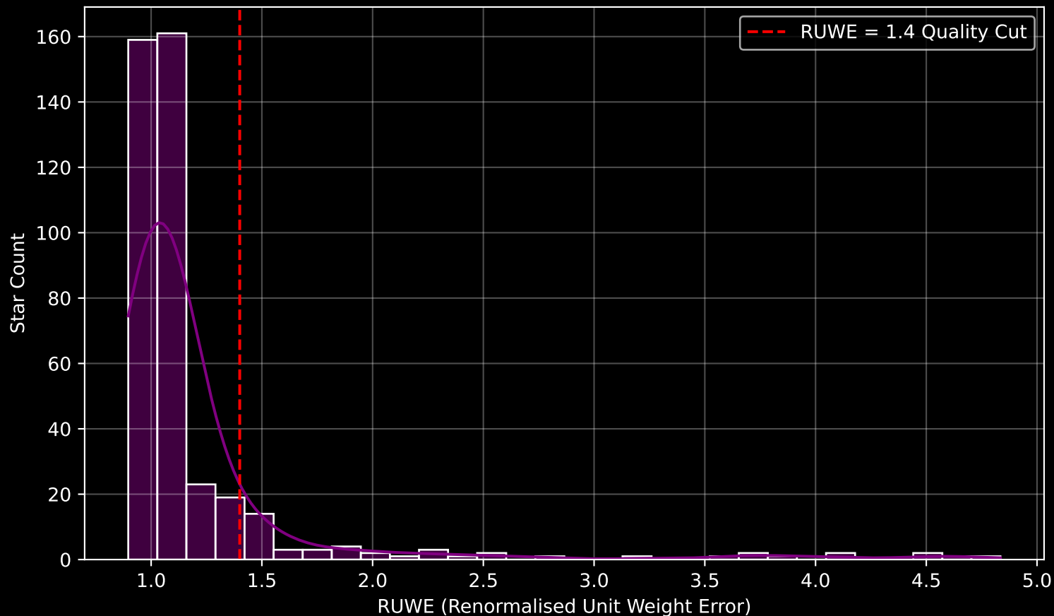
GAPOGEE DR17 Field [300+75] RUWE Distribution (n= 407)
