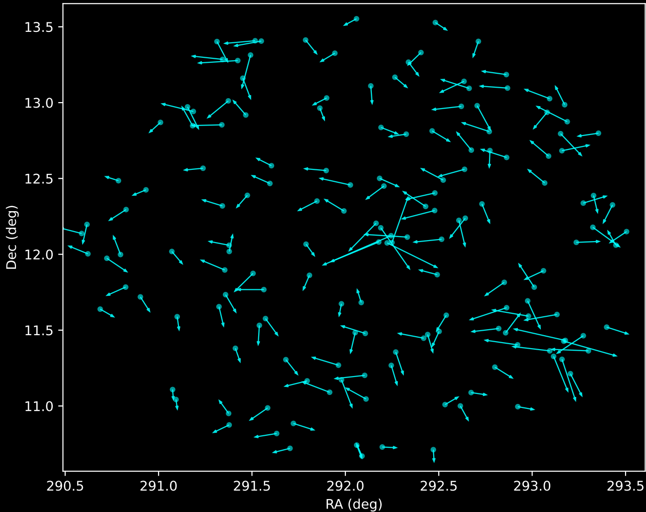
APOGEE DR17 Noise Stream Proper Motion Vectors (n=160)
