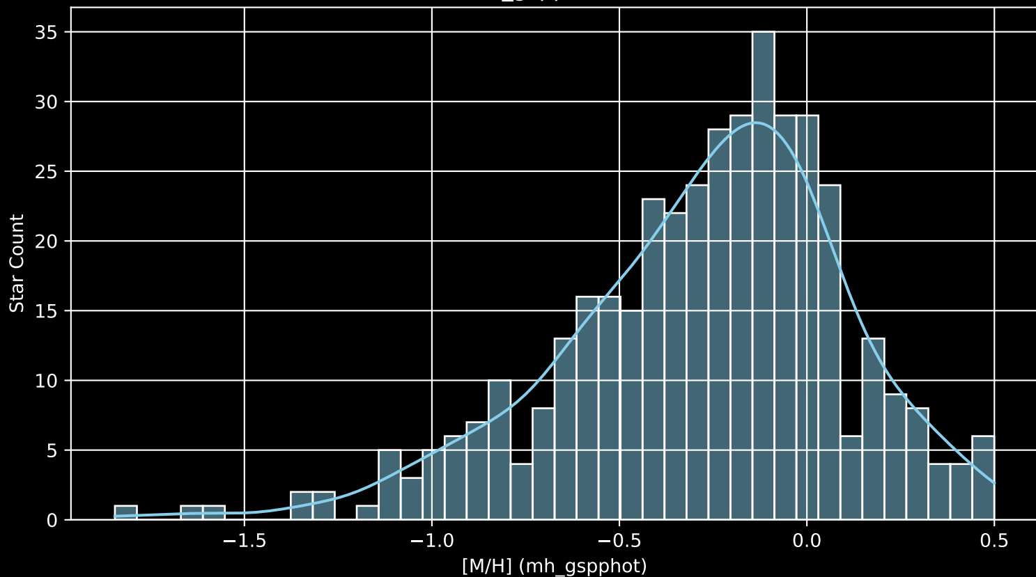
APOGEE DR17 Field: [300+75 [M/H] (mh_gspphot) (n= 409)
