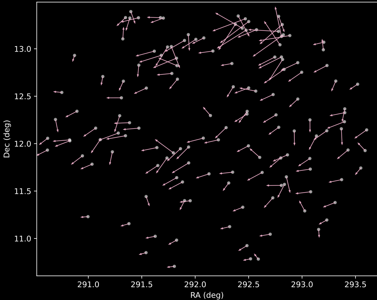
APOGEE DR17 Cluster 13 Proper Motion Vectors (n=138)
