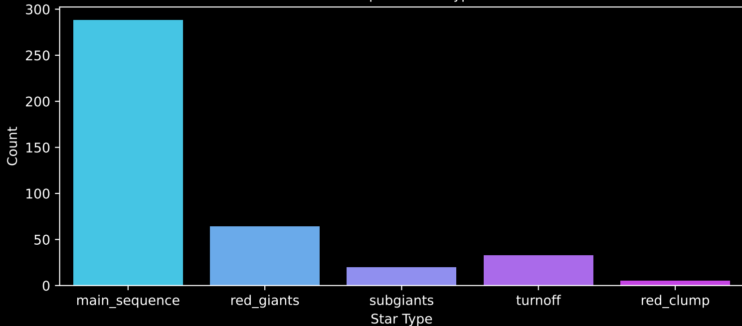
APOGEE DR17 Field: [300+75] Count plot of Star Type
