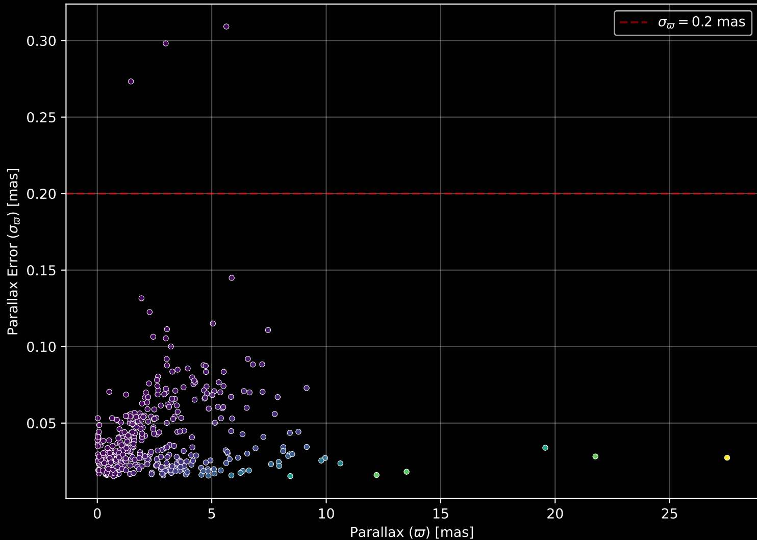
APOGEE DR17 Field: [300+75] Parallax Quality (n= 410)
